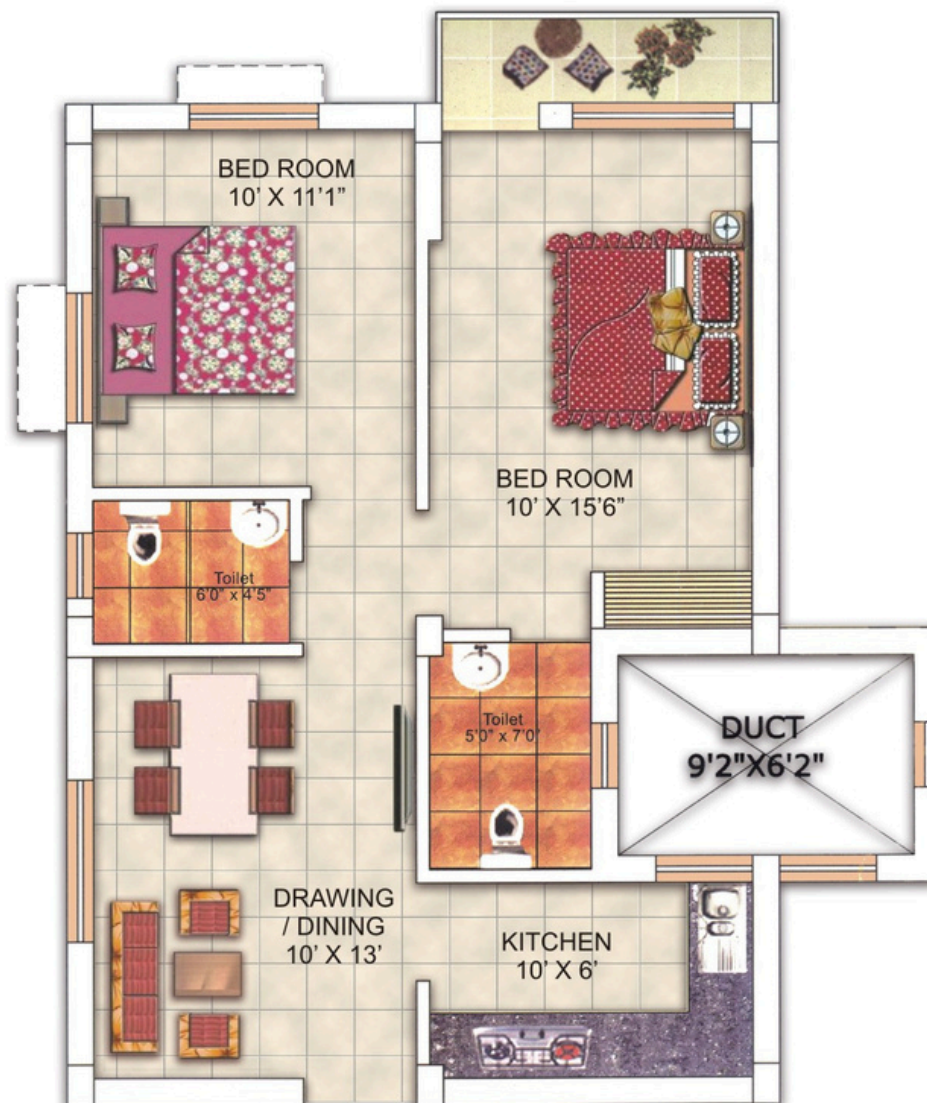
2 BED ROOM FLAT S.B.AREA: 936 sq.ft.
